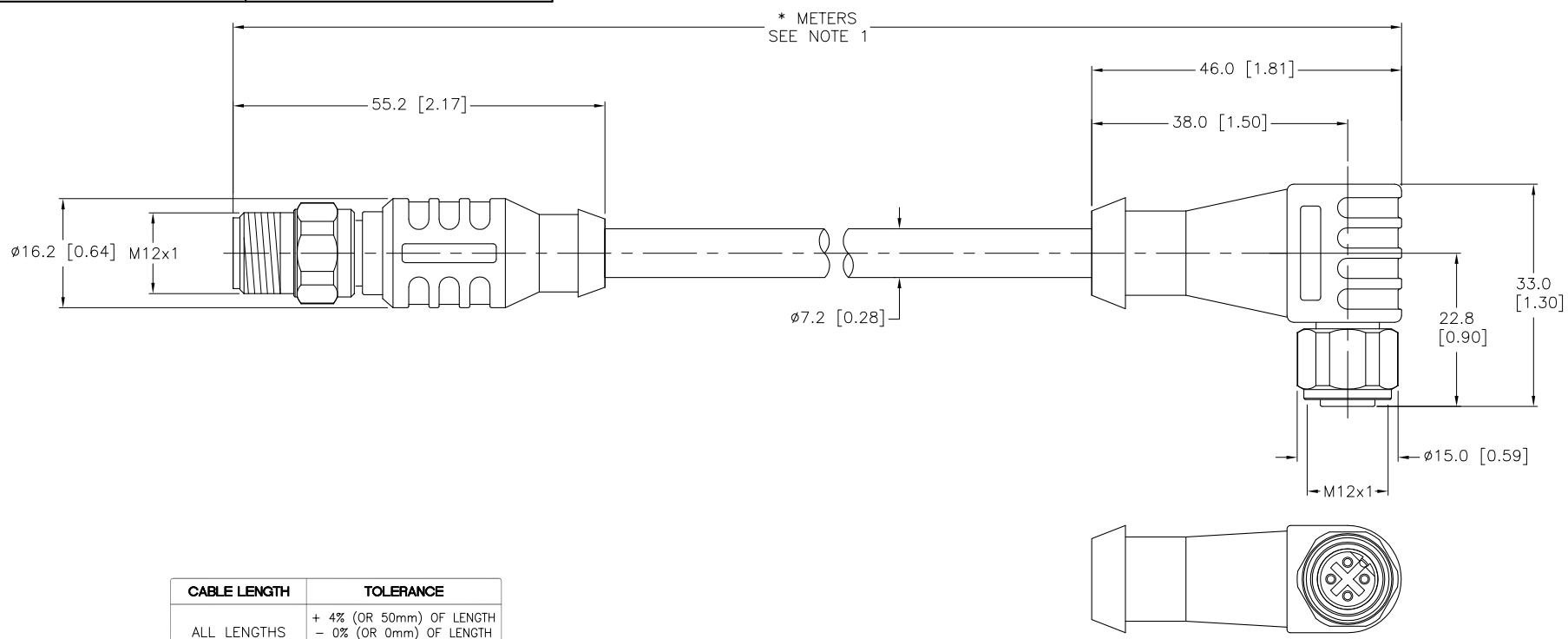
SOURCE DRAWING - FOR REFERENCE ONLY
